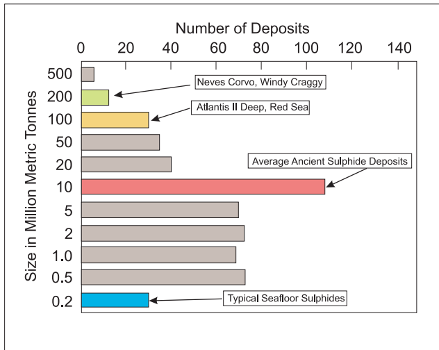
FIG. 8. Worldwide size distribution for VMS deposits, with deposits over 50 Mt considered "giant", and those over 150 Mt considered "supergiant". Atlantis Deep is considered the largest modern example of a seafloor massive sulphide deposit, with Neves Corvo and Windy Craggy ancient examples of supergiant deposits. Modified from Hannington et al (1995).
