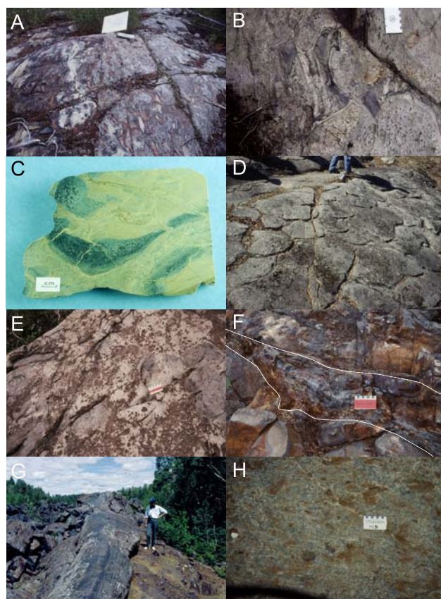
Fig. 16 A) High temperature hydrothermal alteration of mafic volcanoclastic turbidite overlain by a strongly silicified mafic debris flow 1200m below the Chisel-Lost-Ghost VMS horizon, Snow Lake. This represents a regional-scale reaction zone overlain by high temperature zone of silica dumping ; B) Strongly silicified pillows with pipe vesicles infilled with actinolite, epidote and magnetite, and interpillow hyaloclastite completely replaced by the same assemblage. This alteration facies directly overlies the subvolcanic Mooshla intrusion, Bousquet VMS camp; C) An example of epidote typical of the root zones of VMS hydrothermal upflow zones in which high fluid/rock ratios has resulted in leaching of lithophile, chalcophile and LFSE from the strata (J. Lydon); D) Strongly Mg-altered pillows metamorphosed to c.g. anthophyllite-cordierite in the footwall strata to the Winston Lake Zn-Cu deposit, Terrace Bay ON; E) Silicified basaltic andesite of the Upper Amulet fm., Noranda, as an example of pervasive silica dumping that occurs in mafic flows directly underlying tuffaceous exhalite units in many Precambrian VMS camps; F) Mine Contact Tuff exhalite horizon (between white lines) that overlies the silicified andesites of the Waite fm., Noranda; G) Banded magnetite-chert Fe-formation overlying the Austin Brook massive sulphide deposit, Bathurst camp (J. Peter); H) Chloritoid-rich zone below the Matabi deposit, Sturgeon Lake, where Fe-rich hydrothermal fluids crossed a previously-formed carbonate-rich regional alteration zone.
