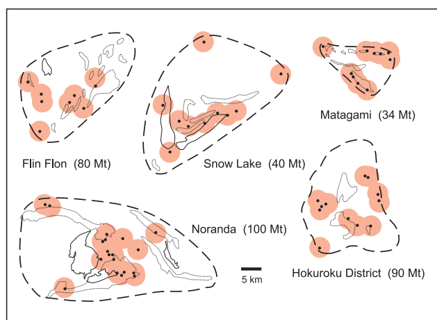
FIG. 12. A same-scale comparison of selected VMS districts. A 5 km diameter circle around each deposit shows the hypothetical area of influence of proximal-scale alteration about each deposit, all encircled by a dashed line defining the proposed extent of a regional-scale alteration system for each camp based on the presence of known felsic volcanic formations. In effect, the Noranda example corresponds closely to the observed alteration. Modified from Sangster (1980).
