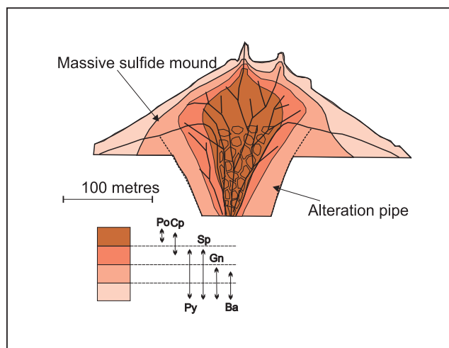
FIG. 19. The mineral zonation commonly observed within VMS deposits is largely a function of hydrothermal fluid temperature and composition. Temperature zonation results in the zoning of sulphide minerals within both the discordant stockwork zone and the conformable sulphide mound. From Lydon (1984).
